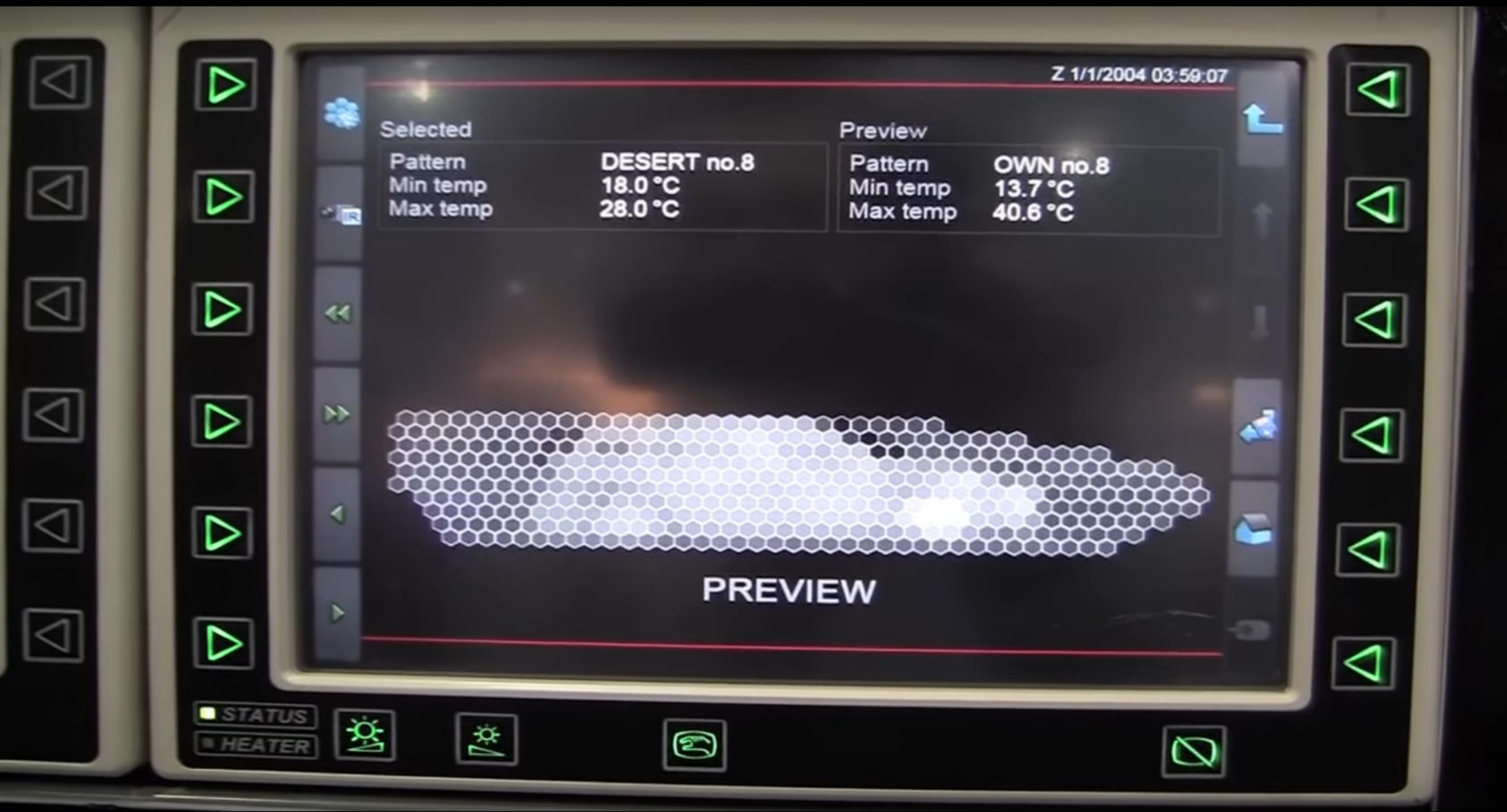
BAE Systems' Adaptiv infra-red 'invisibility cloak' for military vehicles
